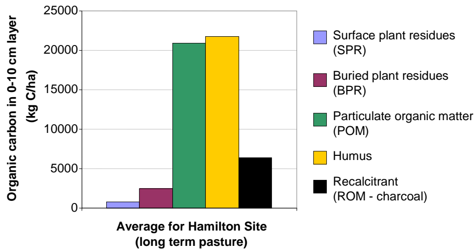
Figure 5: Variation in amount of C associated with soil organic fractions
