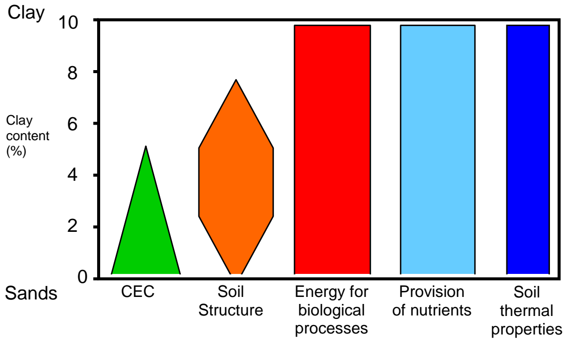
Figure 3: Relationship between the importance of SOM functions and soil type
